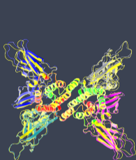
(a) A2B2C2 heteromer TM-score = 98.0, N_{res} = 1,246, PDB ID = 6E3K
