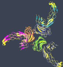
(b) A3B3 heteromer TM-score = 89.3, N_{res} = 795, PDB ID = 7KHD
